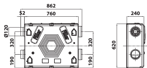
CEILING INSTALLATION
