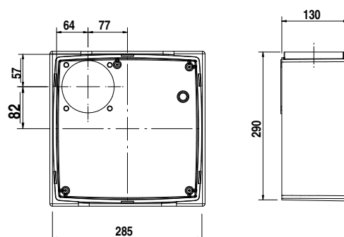
Casing for built-in installation (to be ordered separately)
